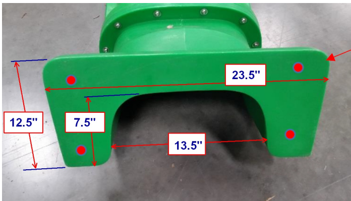
Top Piece mounting flange.
